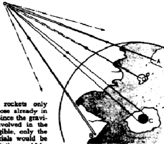
Fig. 2. Typical extra-terrestrial relay services. Transmission from A being relayed to point B and area C; transmission from D being relayed to whole hemisphere.
